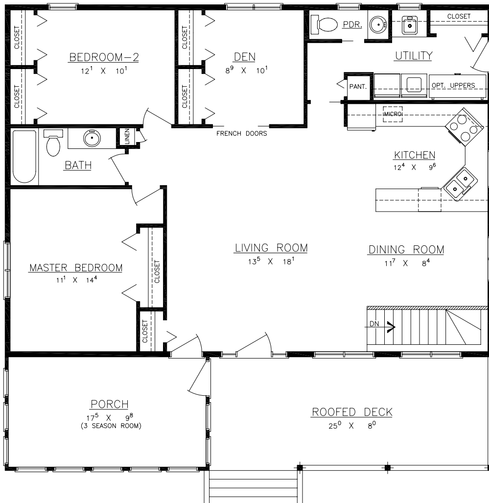
FLOOR PLAN
